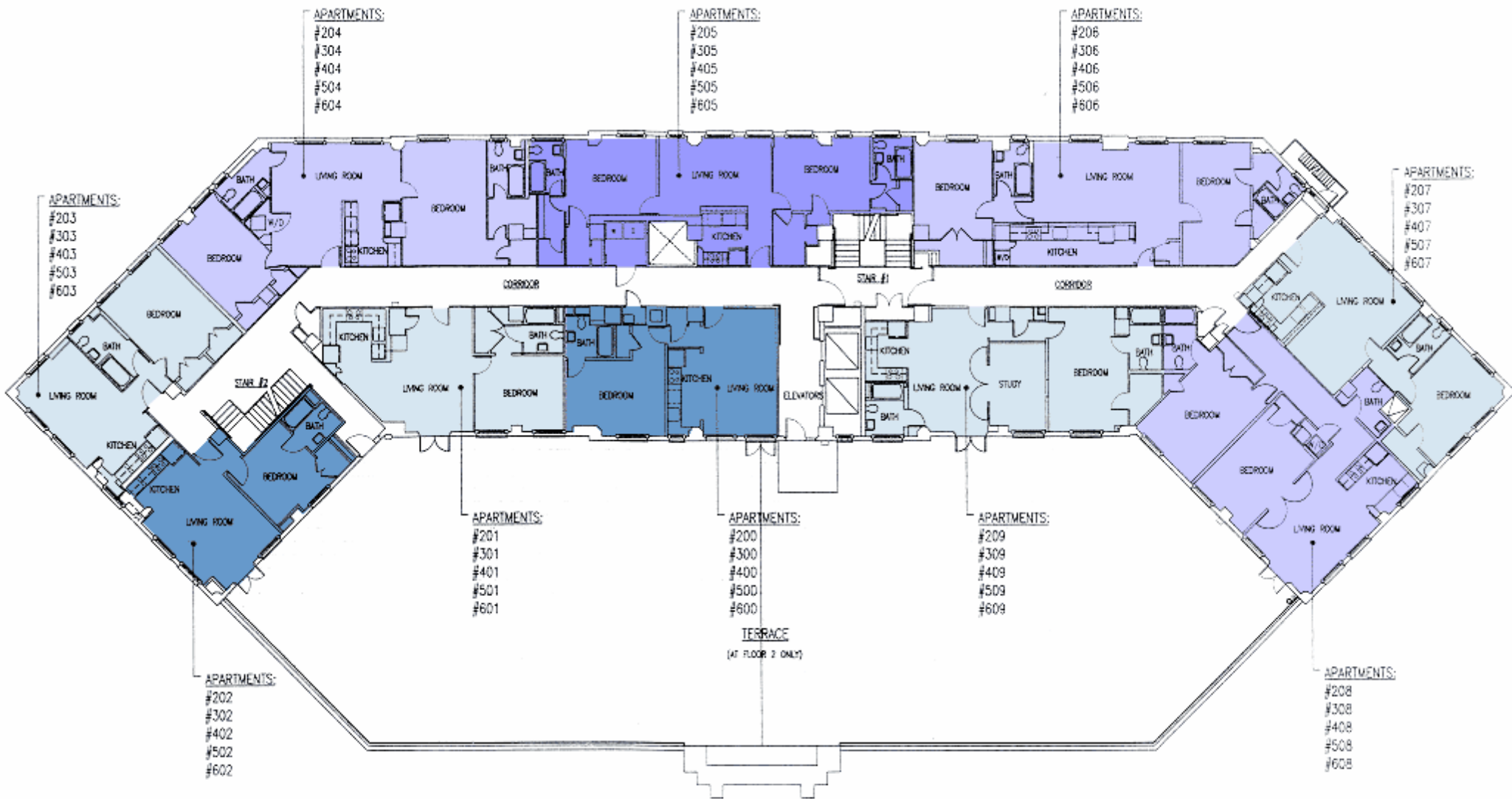
FLOOR PLAN 2nd THRU 6th FLOORS
